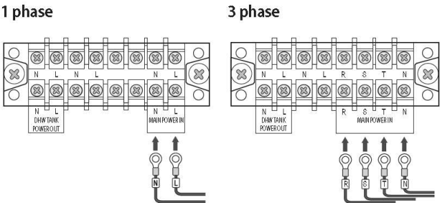
Power wire connection
