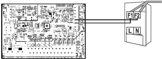
Communication cable connection
