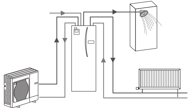
Diagram over kompakt cylindersystem
